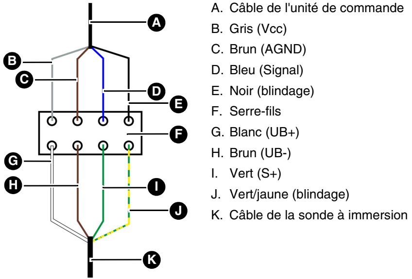
Figure 7: Raccordement serre-fils
