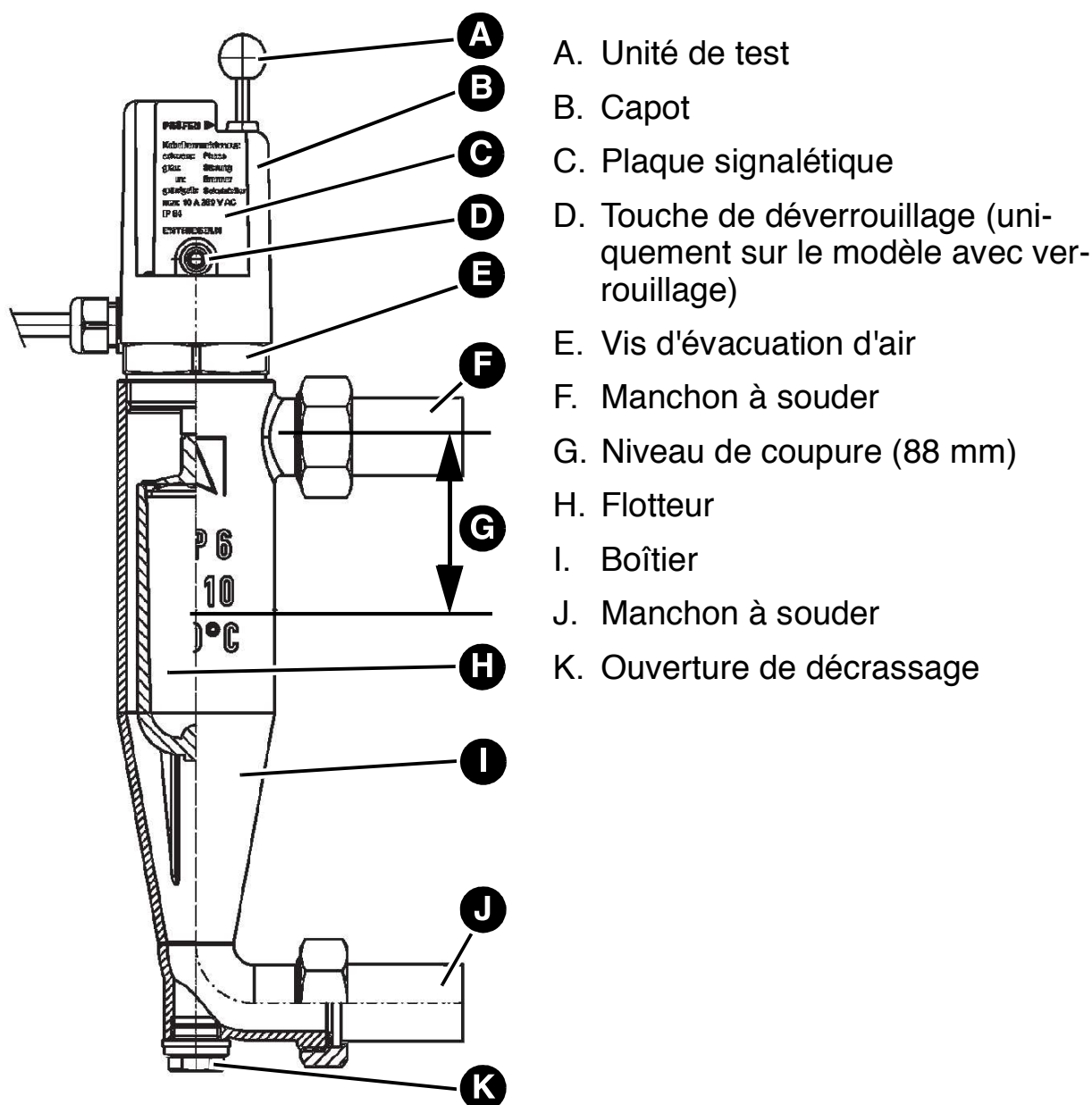
Figure 1: Aperçu WMS-WP6
