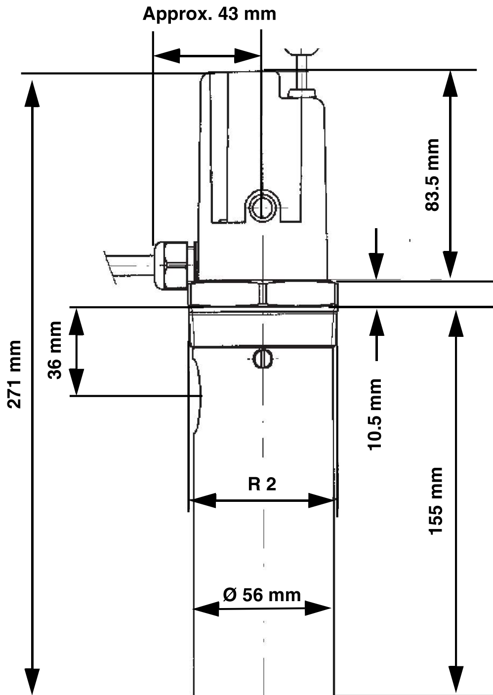
Fig. 4: WMS-WP6 with short protective pipe
