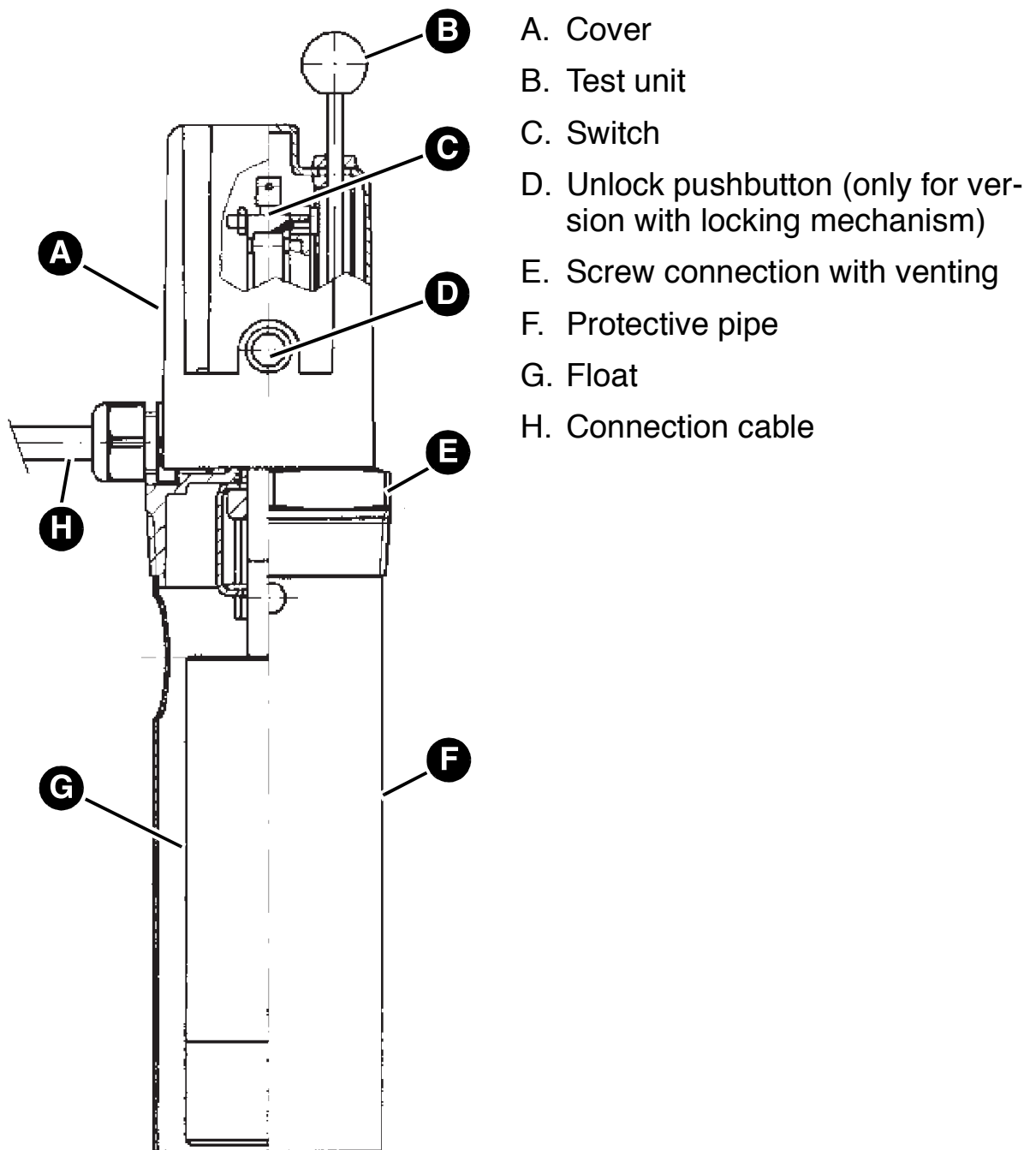
Fig. 2: WMS-WP6 with short protective pipe
