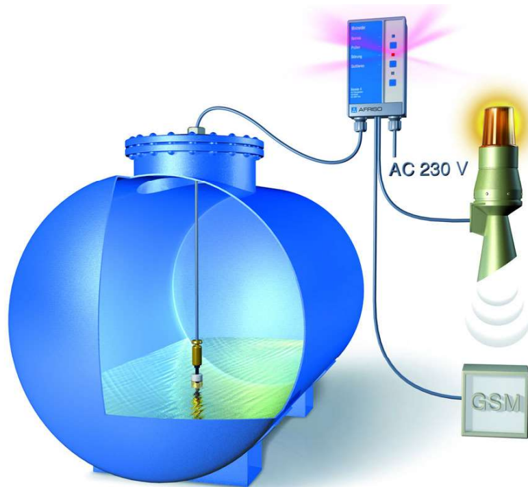
Fig 3: Standard application Minimelder-R
