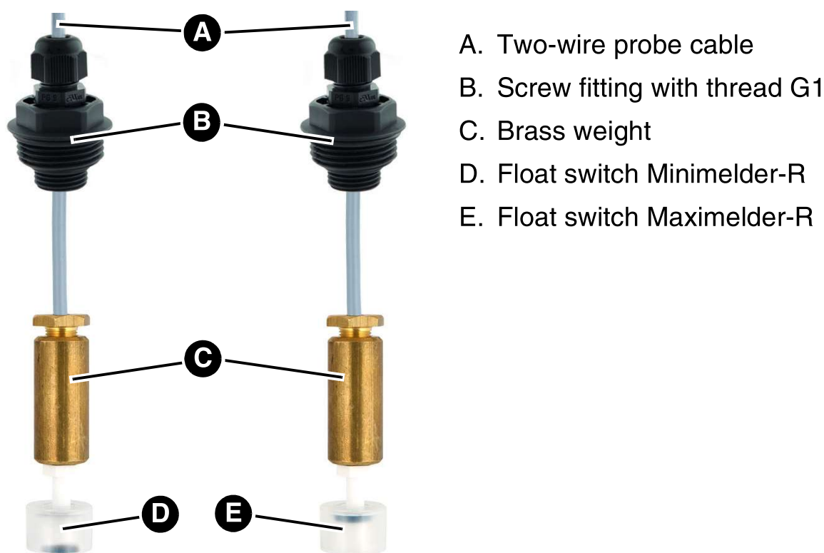
Fig 1: Floating probe
