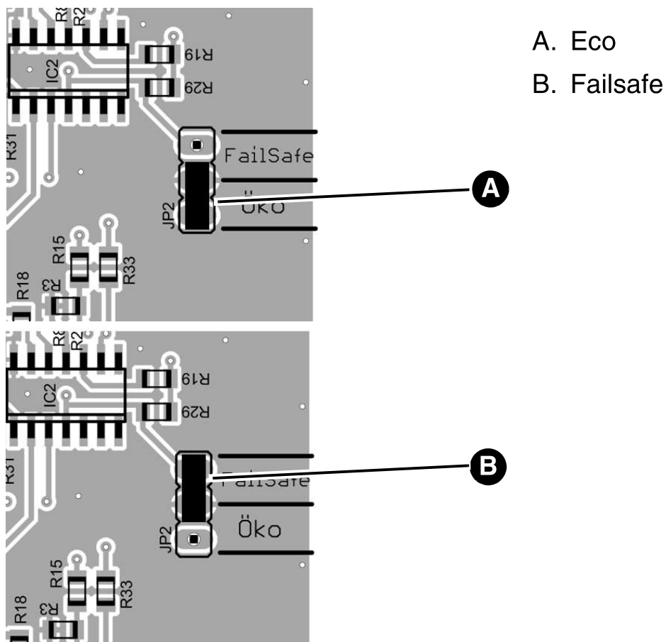
Fig 6: Setting the operating mode
