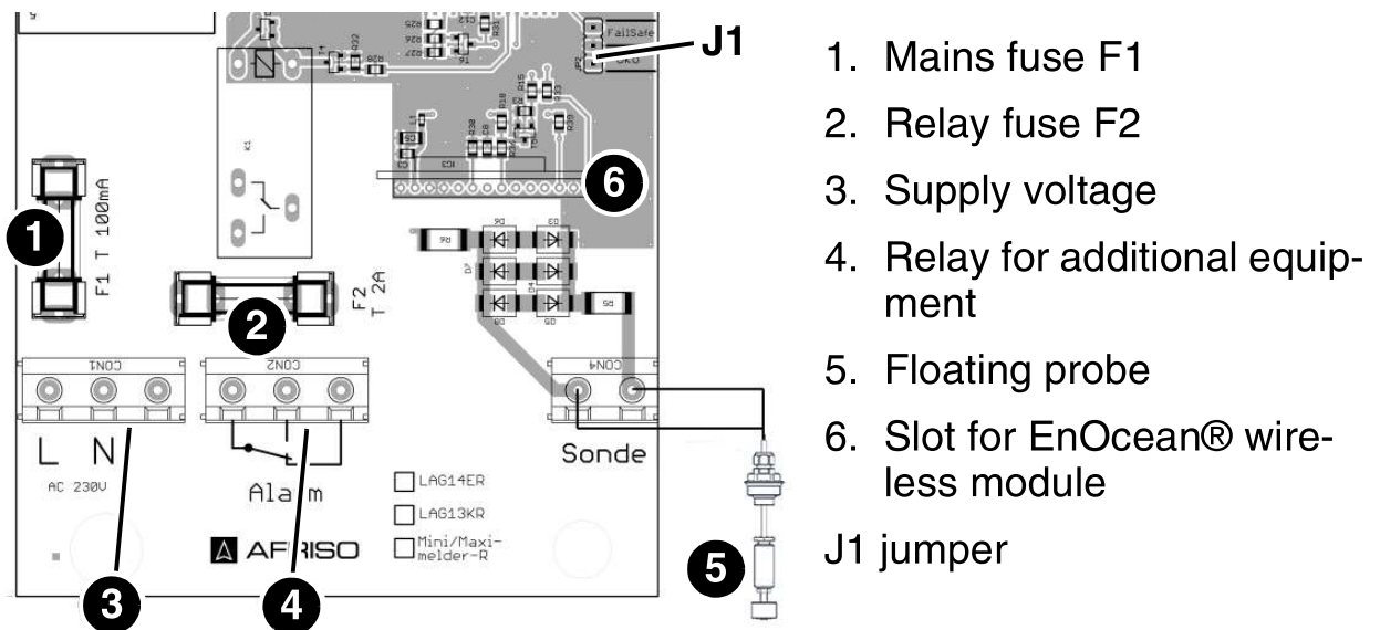
Fig 5: Electrical connection
