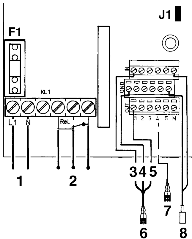
Fig. 7: Electrical connection OM 5+1
