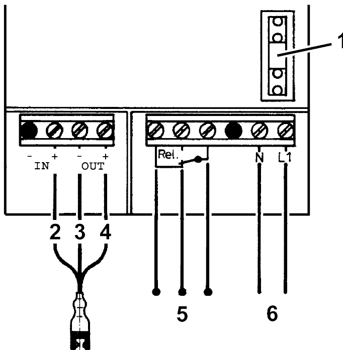
Fig. 8: Electrical connection OM 1
