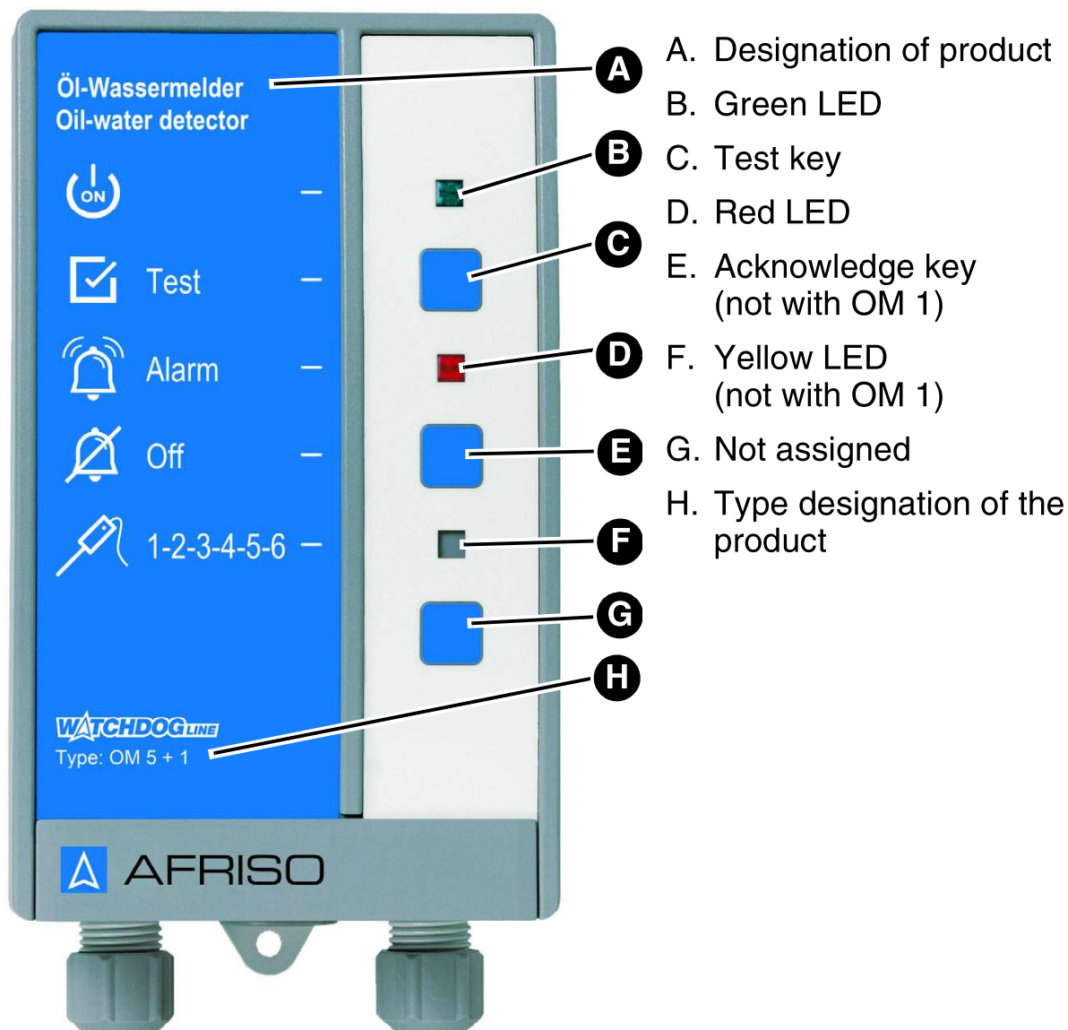
Fig. 3: Control unit
